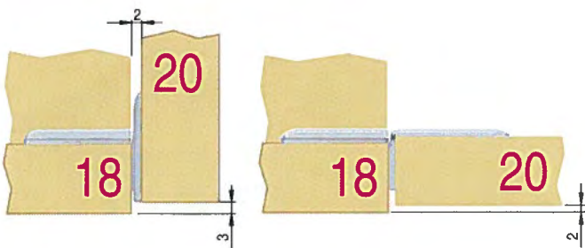
ADAPTOR FOR BOTTOM PANEL 1,5mm VERTICAL ADJUSTMENT +2mm
