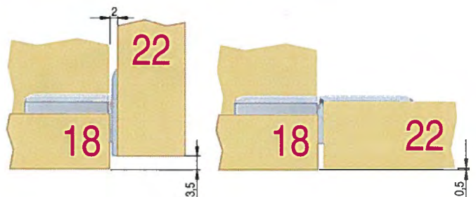
ADAPTOR FOR BOTTOM PANEL 4mm
