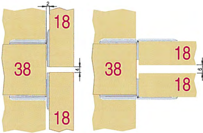
ADAPTOR FOR BOTTOM PANEL 1,5mm
