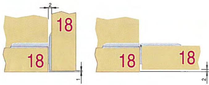
ADAPTOR FOR BOTTOM PANEL 1,5mm
